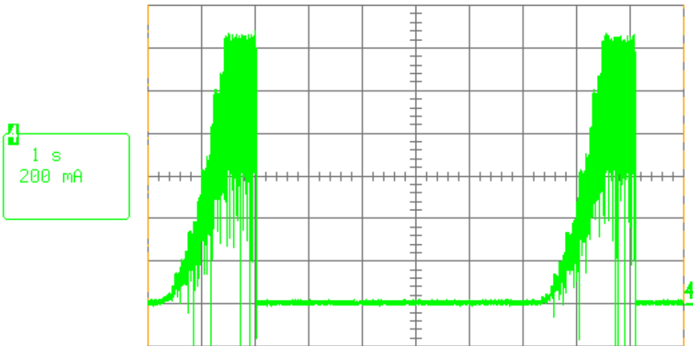
Locked rotor current @ 24 V
