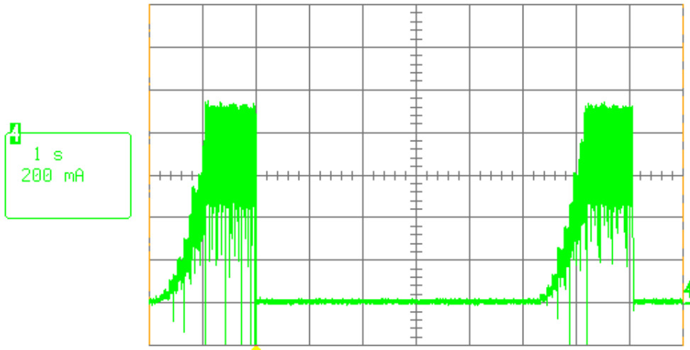
Locked rotor current @ 30 V
