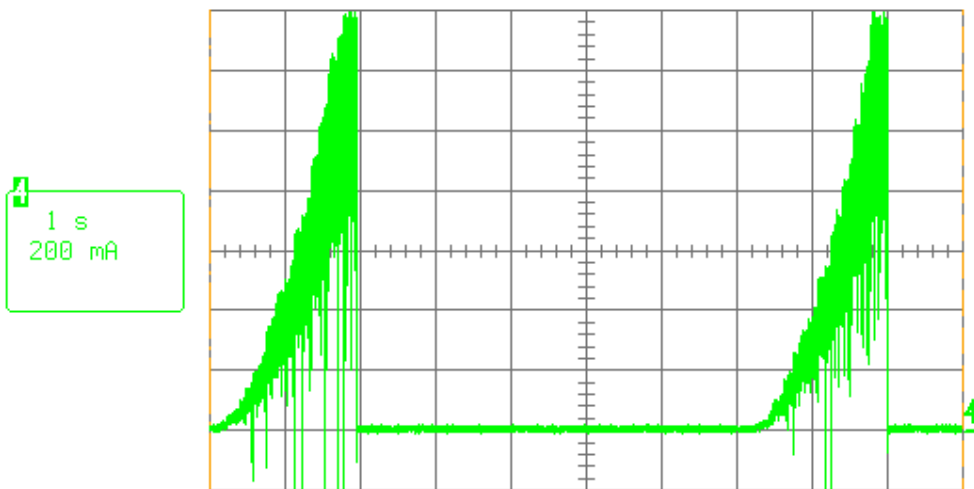
Locked rotor current @ 16 V
