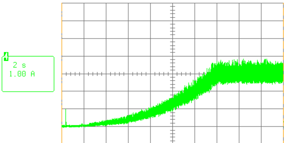
Startup current @ 24 V; 0 - 9.500 1/min
