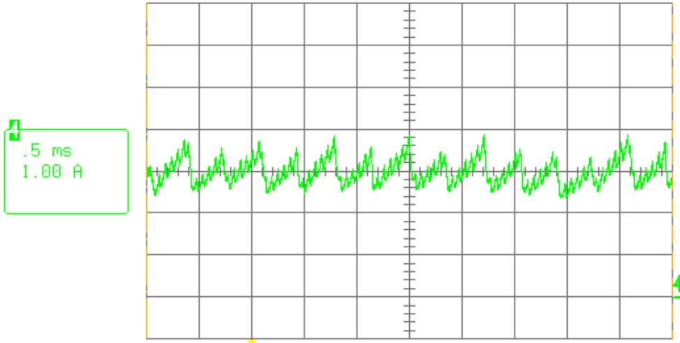
Typical running current @ 24 V - free blowing, 9.500 1/min
