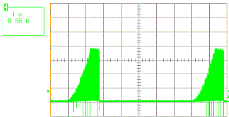
Locked rotor current @ 48 V
