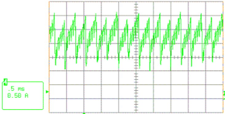
Typical running current @ 48 V, free blowing, 11.000 1/min
