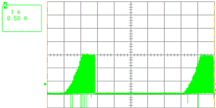
Locked rotor current @ 60 V
