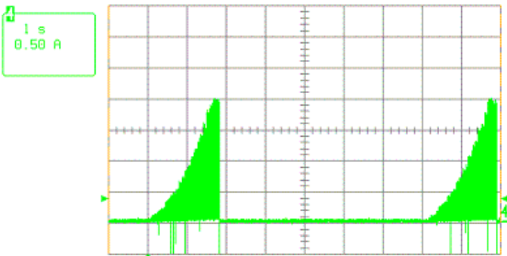
Locked rotor current @ 36 V
