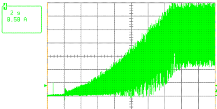
Start-up current @ 48 V, 0 - 11.000 1/min
