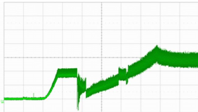
Start-up current @ 12 V ( I = 1\text{A/div} ; t = 2\text{s/div} )
