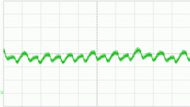
Running current @ 12 V (I = 1A/div ; t = 500ms/div)
