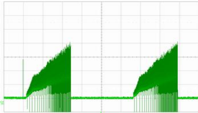
Locked rotor current at 48,0 V; I=500mA/Div, t=1s/Div
