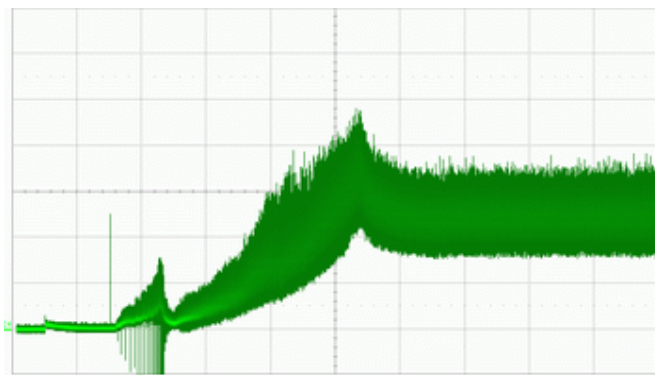
Start-up current at 48,0 V; I=500\text{mA/Div} , t=2\text{s/Div}
