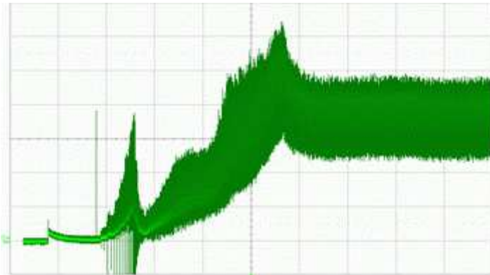
Start-up current @ 48 V ( I = 200\text{mA}/\text{div} ; t = 2\text{s}/\text{div} )
