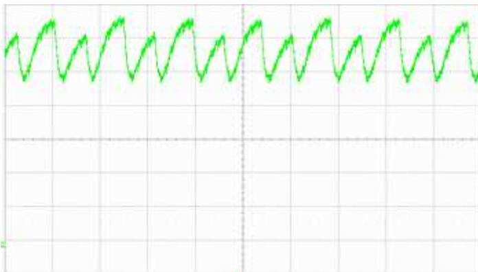
Running current @ 24 V ( I = 1\text{A/div} ; t = 500\mu\text{s/div} )
