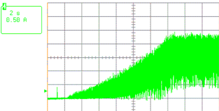
Startup current @ 48V; 0 - 9500 rpm
