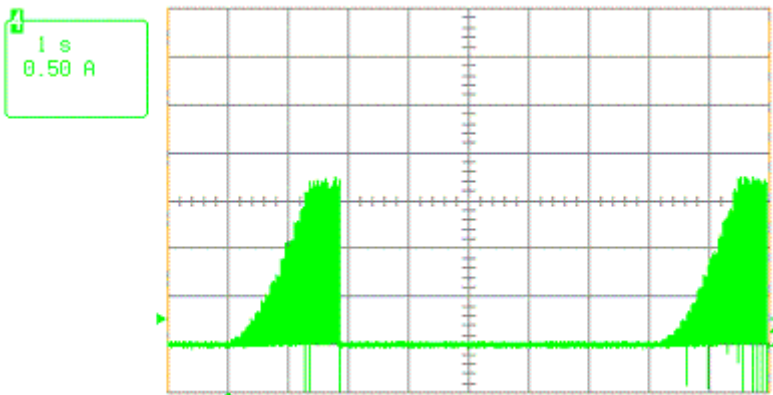
Locked rotor current @ 48V
